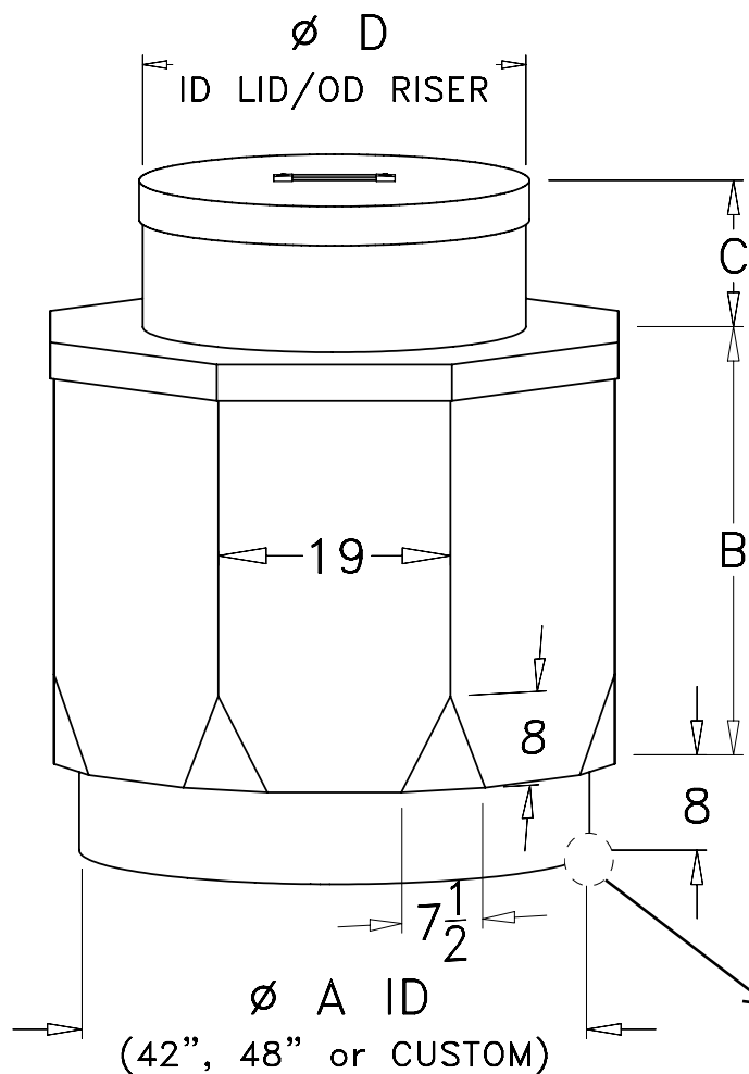
DOUBLE WALL DETAIL
