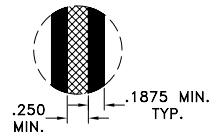
DOUBLE WALL DETAIL
